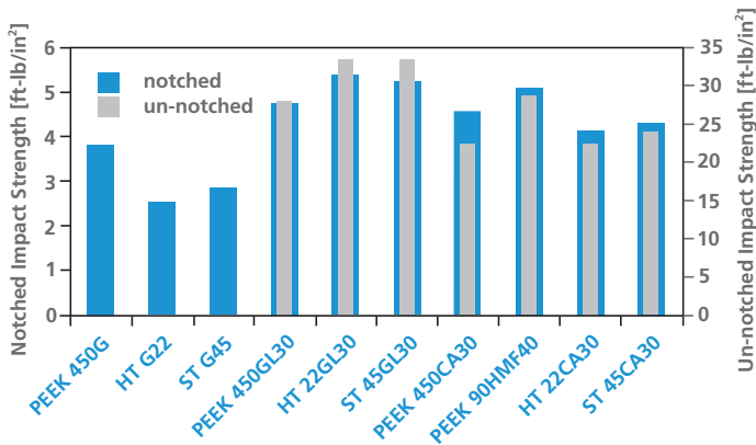
Figure 10: Izod impact strength of various Victrex materials at 73°F
